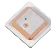
GPS SDARS PAGES-14F2P2G-xxx-xxx GPS: 25x25x4mm SDARS: 36x36x4mm
