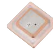
L1 L2 PADGPS-I4H4G-xxx-xxx L1: 25x25x4mm L2: 36x36x4mm 38x38x4mm
